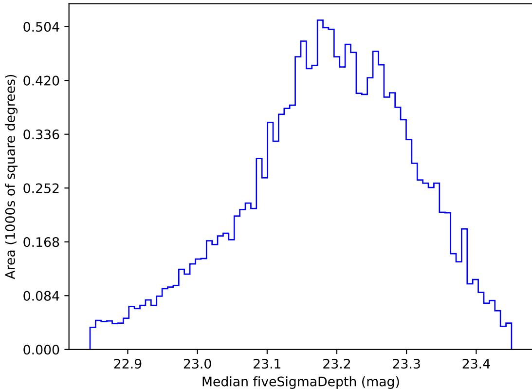
too_elab_r256_d2_ugrizy_v3.4_10yrs WFD u band: Median fiveSigmaDepth
