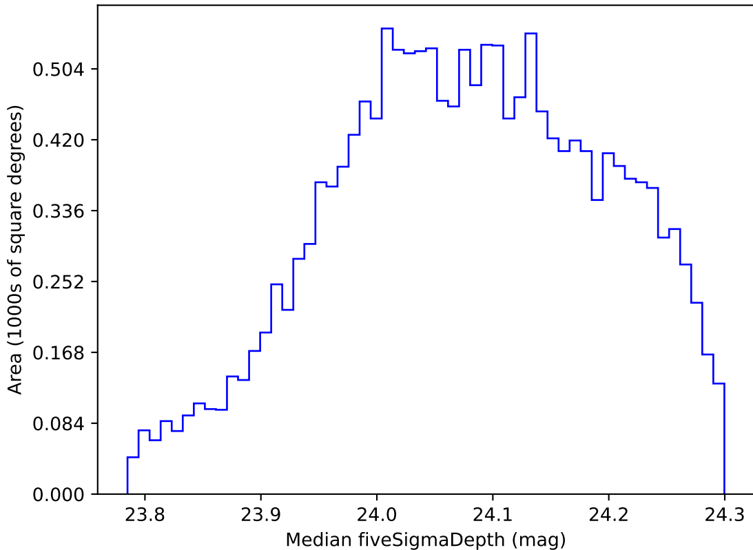
too_elab_r256_d2_ugrizy_v3.4_10yrs WFD r band: Median fiveSigmaDepth
