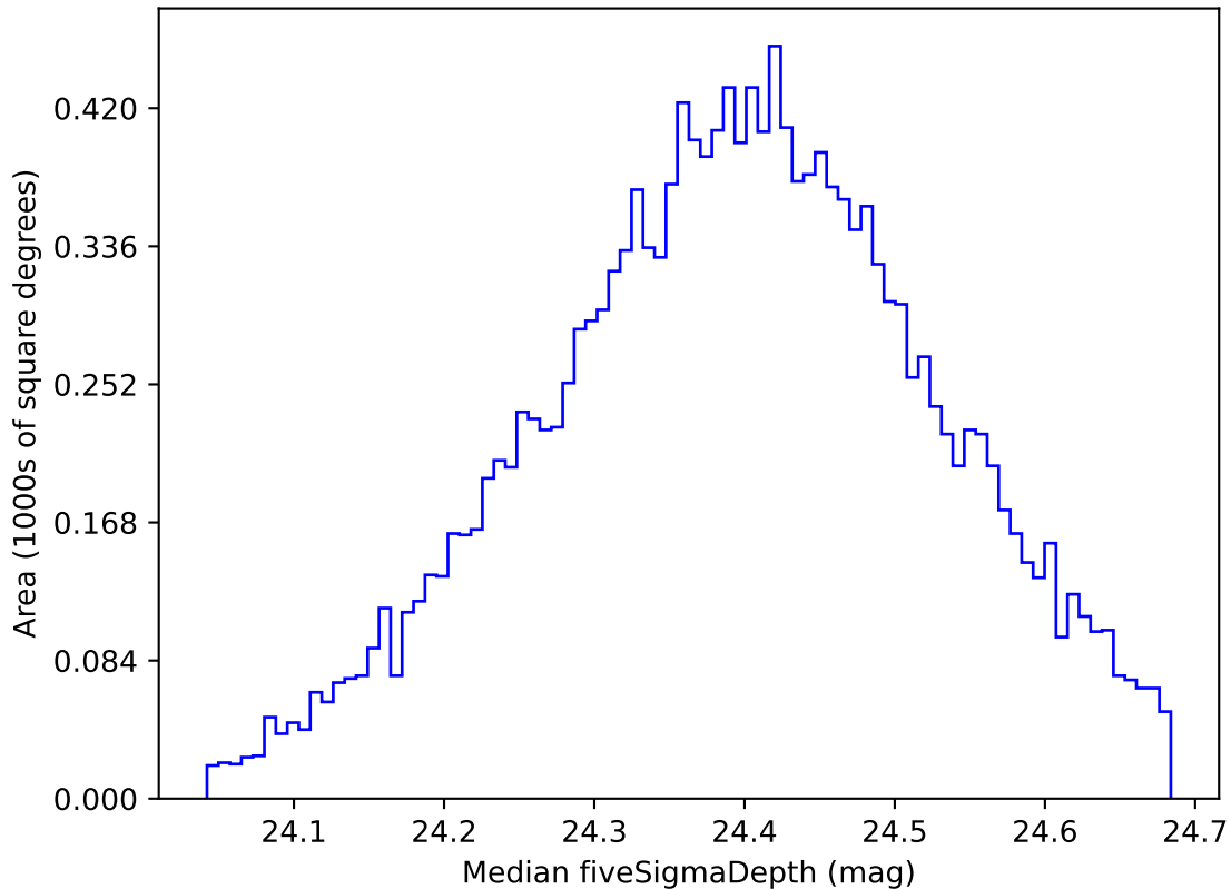
too_elab_r256_d2_ugrizy_v3.4_10yrs WFD g band: Median fiveSigmaDepth
