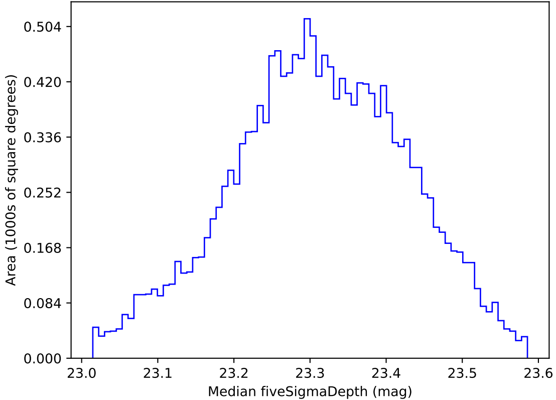
too_elab_r256_d2_ugrizy_v3.4_10yrs WFD all bands: Median fiveSigmaDepth
