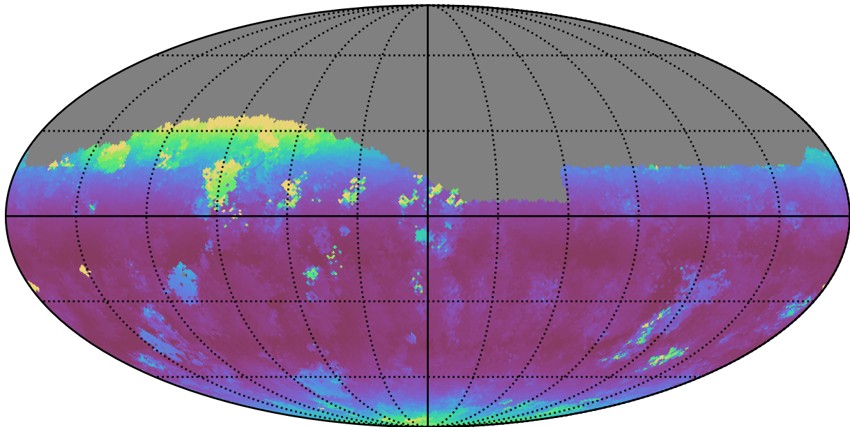
too_elab_r256_d2_ugrizy_v3.4_10yrs Yr 1 z band: Median airmass
