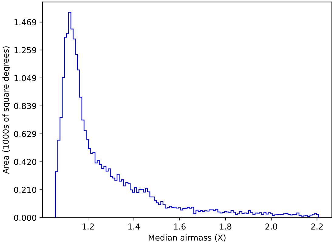
too_elab_r256_d2_ugrizy_v3.4_10yrs Yr 1 z band: Median airmass
