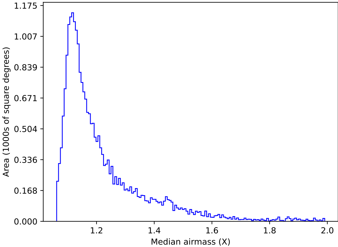
too_elab_r256_d2_ugrizy_v3.4_10yrs Yr 1 y band: Median airmass
