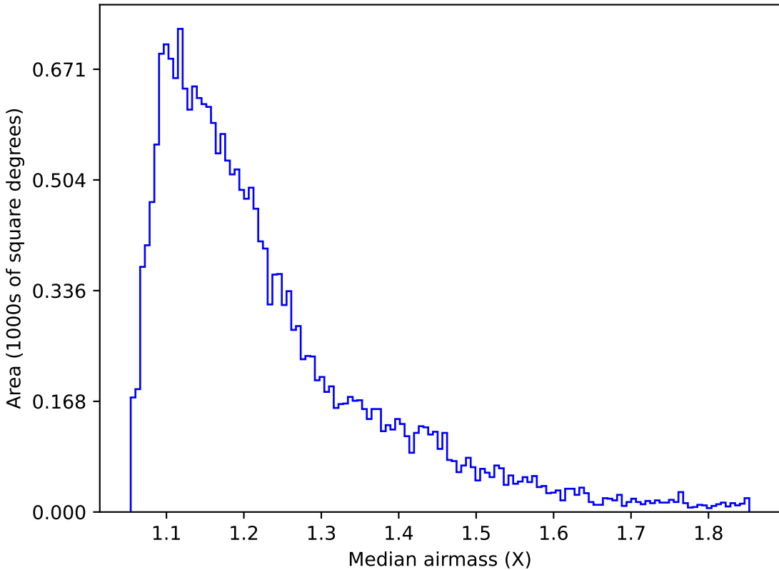
too_elab_r256_d2_ugrizy_v3.4_10yrs Yr 1 u band: Median airmass
