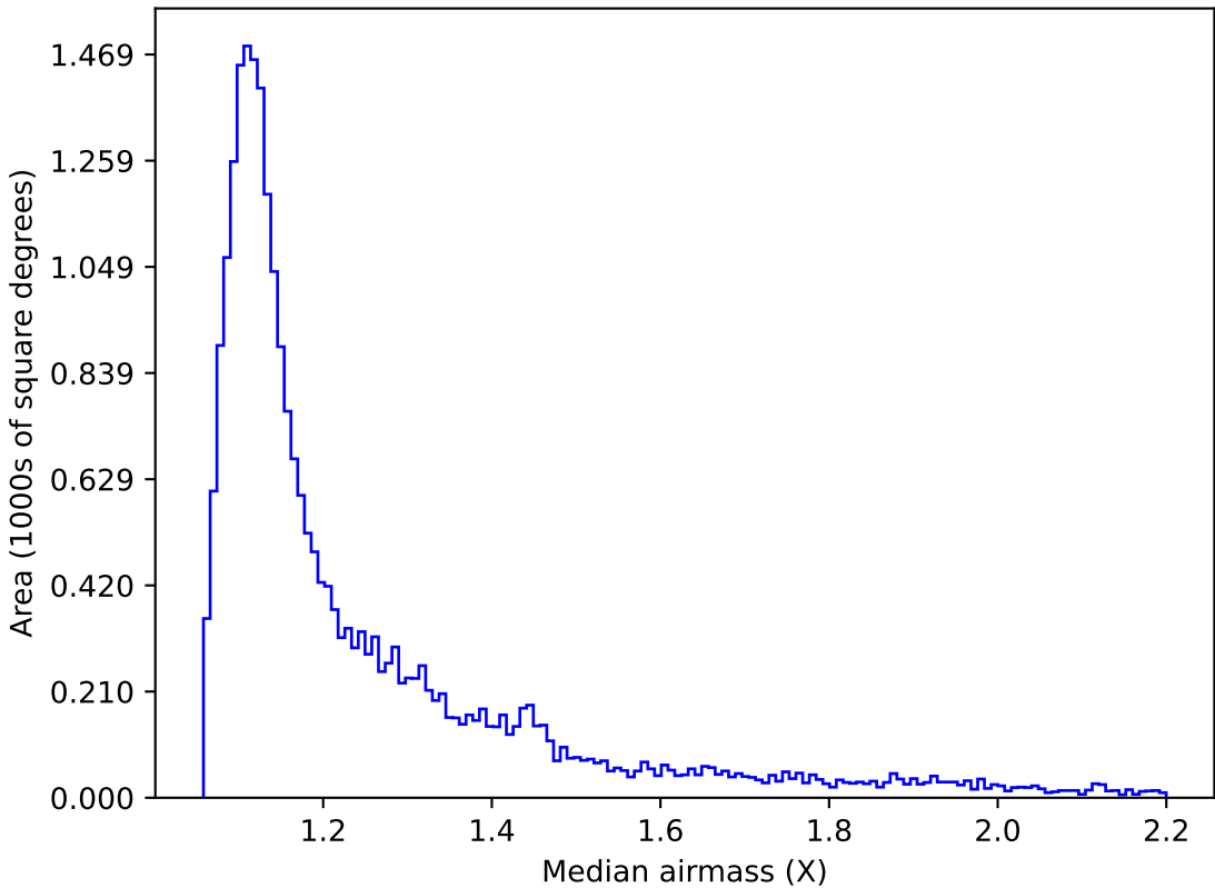
too_elab_r256_d2_ugrizy_v3.4_10yrs Yr 1 i band: Median airmass
