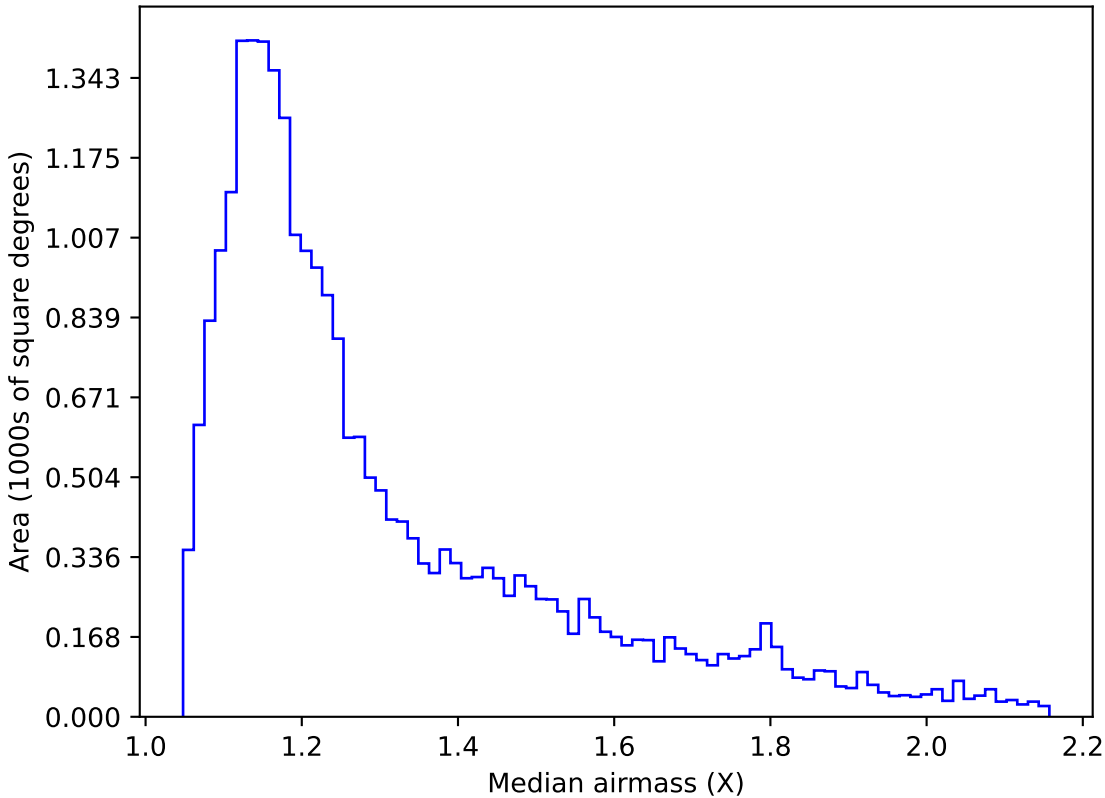
too_elab_r256_d2_ugrizy_v3.4_10yrs Yr 1 g band: Median airmass
