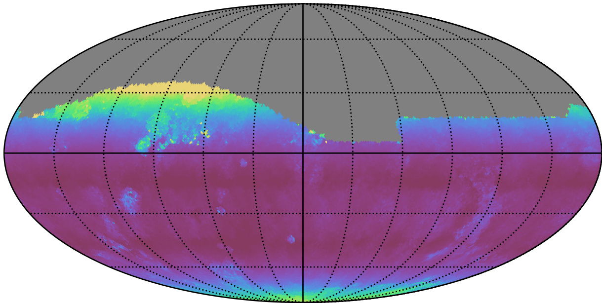
too_elab_r256_d2_ugrizy_v3.4_10yrs Yr 1 all bands: Median airmass
