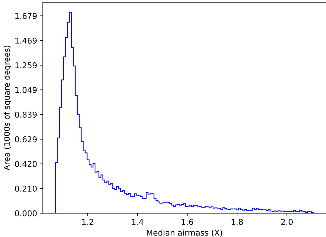
too_elab_r256_d2_ugrizy_v3.4_10yrs Yr 1 all bands: Median airmass
