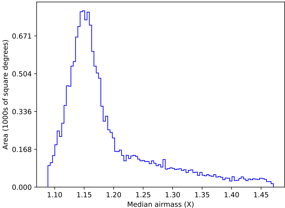
too_elab_r256_d2_ugrizy_v3.4_10yrs WFD z band: Median airmass
