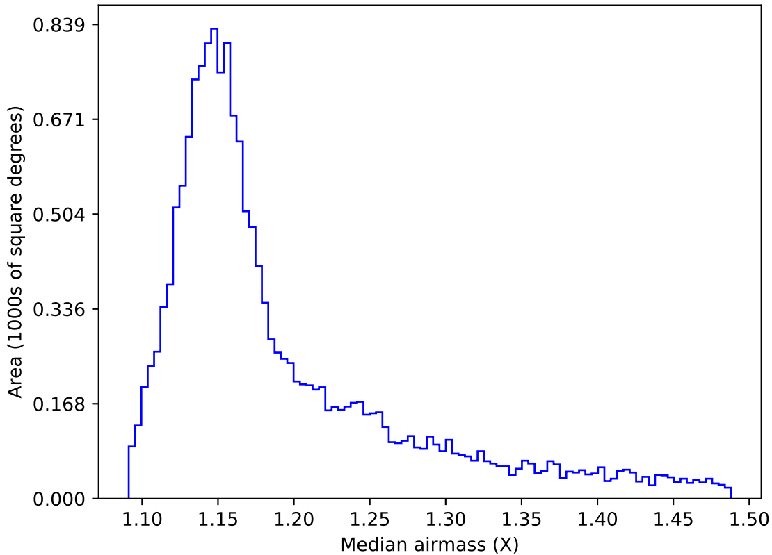
too_elab_r256_d2_ugrizy_v3.4_10yrs WFD y band: Median airmass
