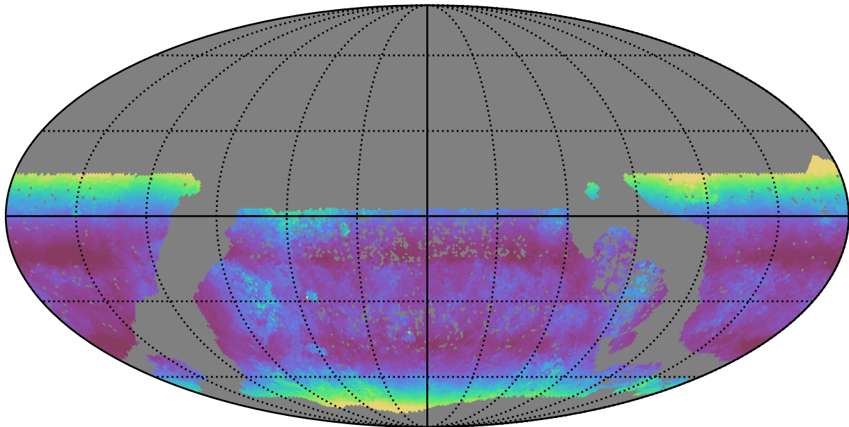
too_elab_r256_d2_ugrizy_v3.4_10yrs WFD u band: Median airmass
