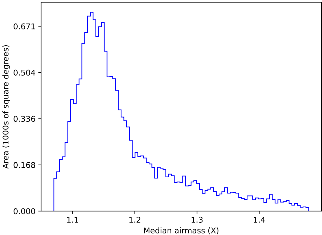
too_elab_r256_d2_ugrizy_v3.4_10yrs WFD u band: Median airmass
