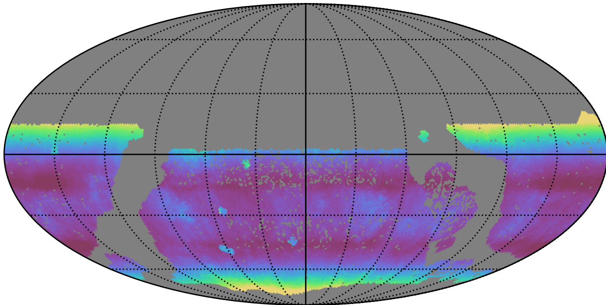
too_elab_r256_d2_ugrizy_v3.4_10yrs WFD r band: Median airmass
