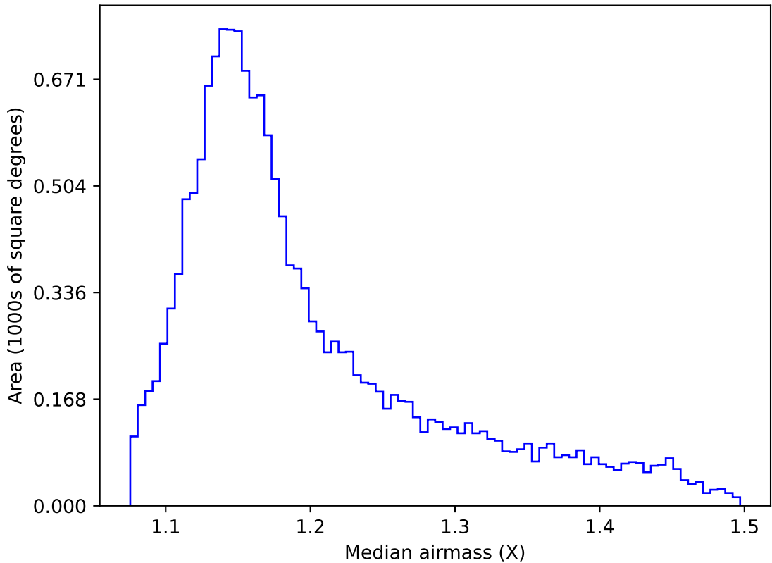
too_elab_r256_d2_ugrizy_v3.4_10yrs WFD g band: Median airmass
