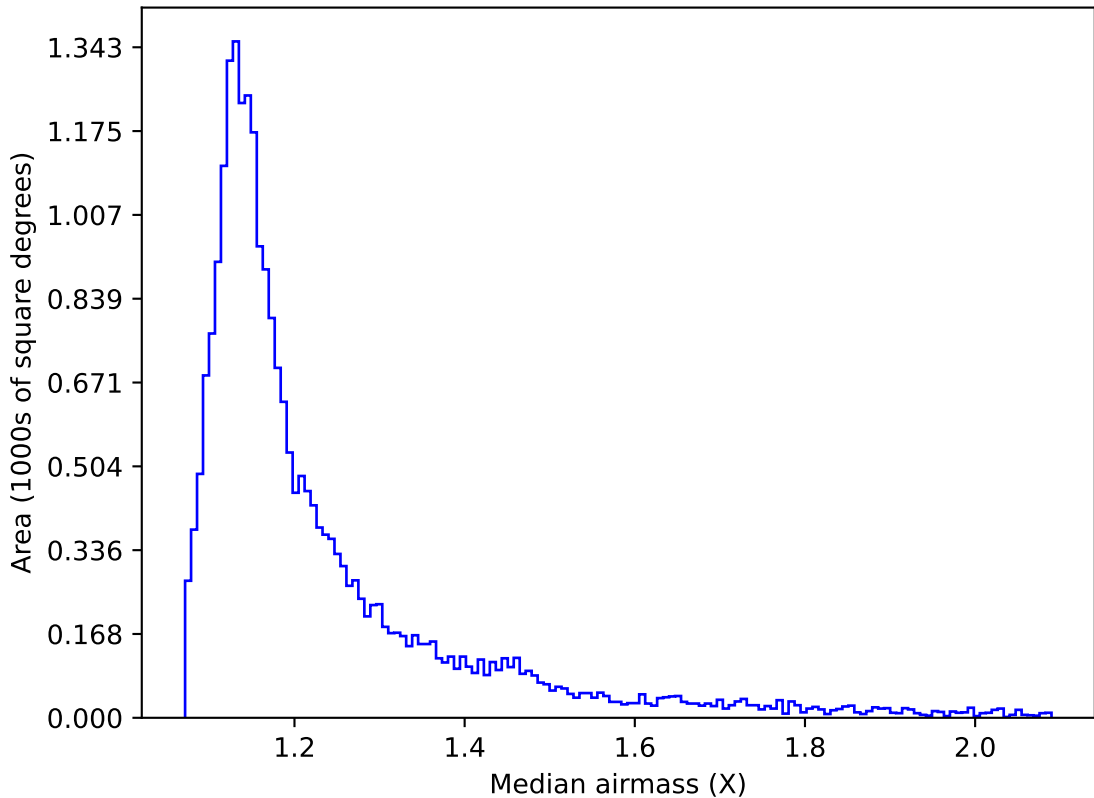
too_elab_r256_d2_ugrizy_v3.4_10yrs All sky u band: Median airmass
