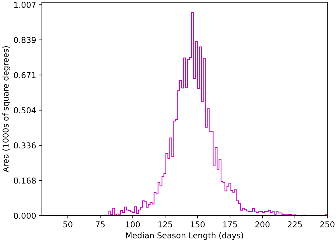
too_elab_r256_d2_ugrizy_v3.4_10yrs WFD z band: Median Season Length
