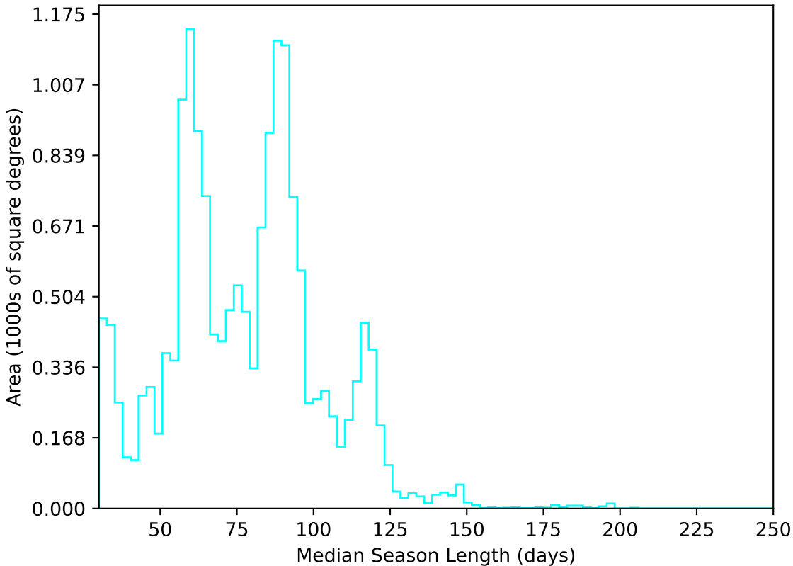
too_elab_r256_d2_ugrizy_v3.4_10yrs WFD u band: Median Season Length
