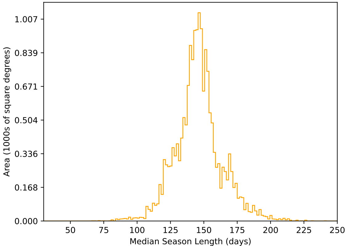
too_elab_r256_d2_ugrizy_v3.4_10yrs WFD r band: Median Season Length
