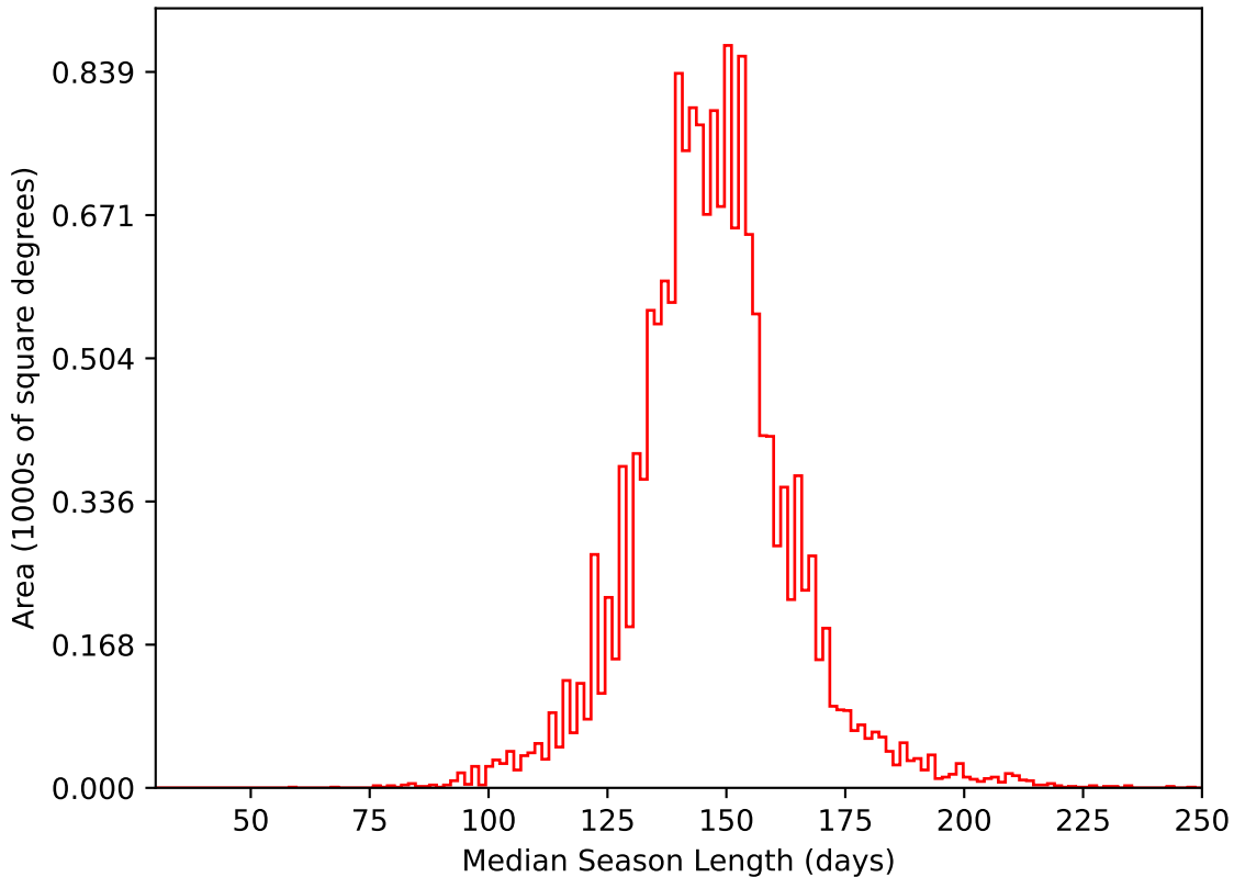
too_elab_r256_d2_ugrizy_v3.4_10yrs WFD i band: Median Season Length
