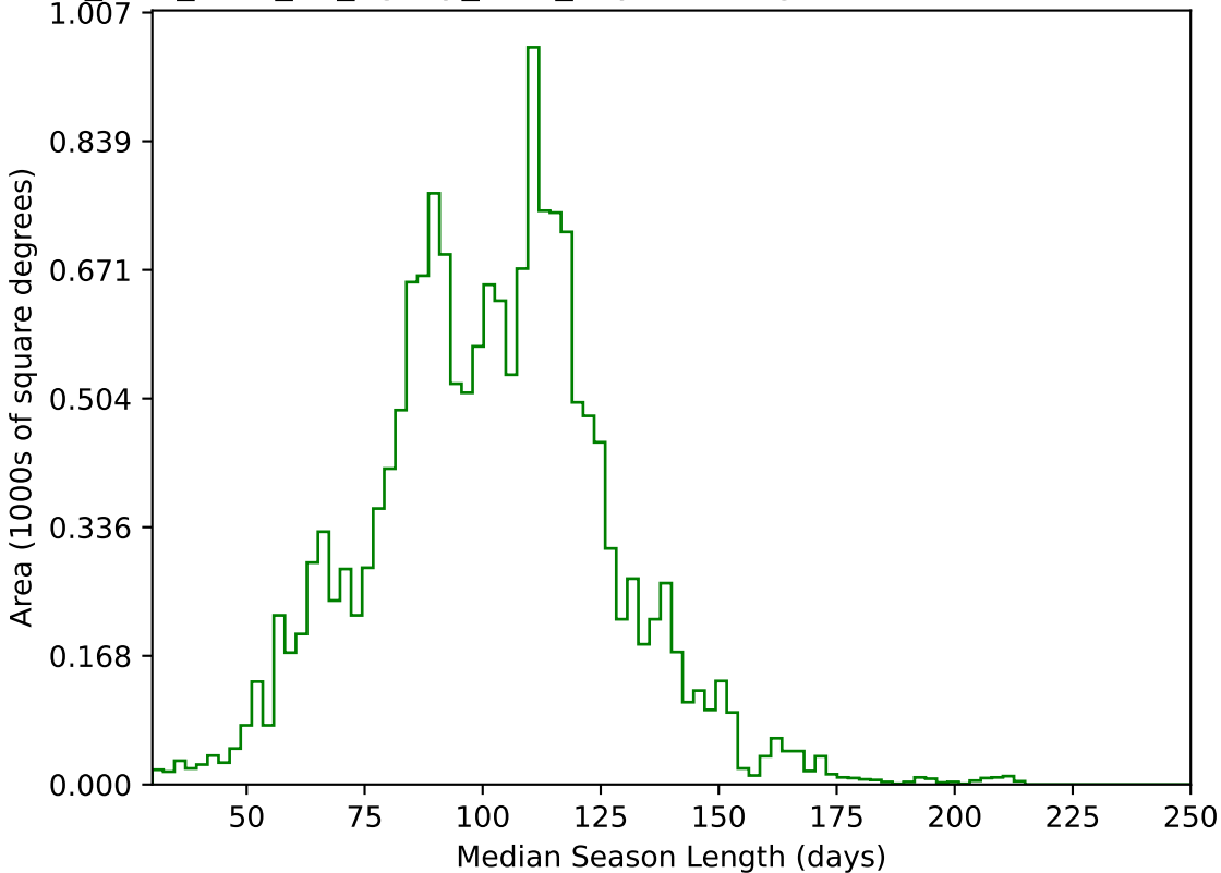
too_elab_r256_d2_ugrizy_v3.4_10yrs WFD g band: Median Season Length
