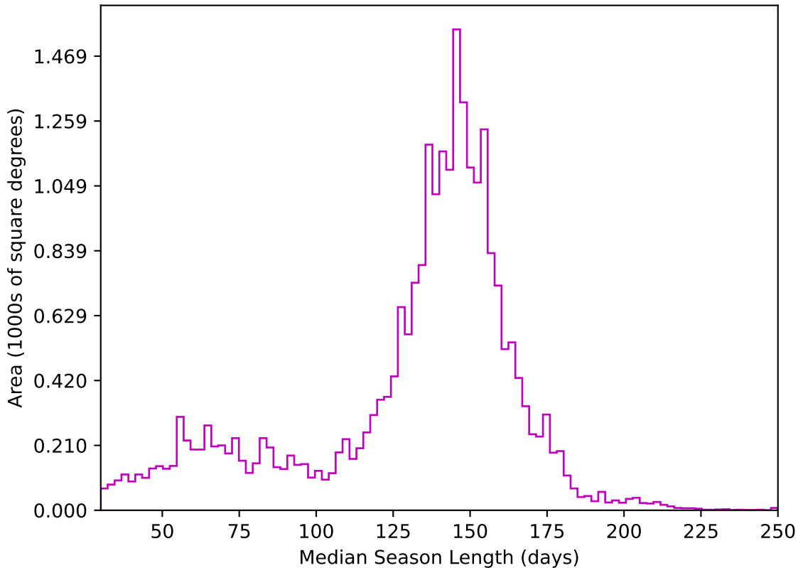
too_elab_r256_d2_ugrizy_v3.4_10yrs All sky z band: Median Season Length
