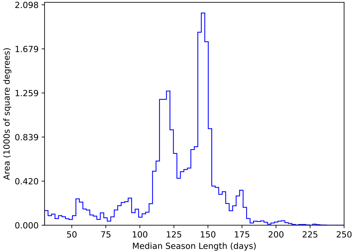
too_elab_r256_d2_ugrizy_v3.4_10yrs All sky y band: Median Season Length
