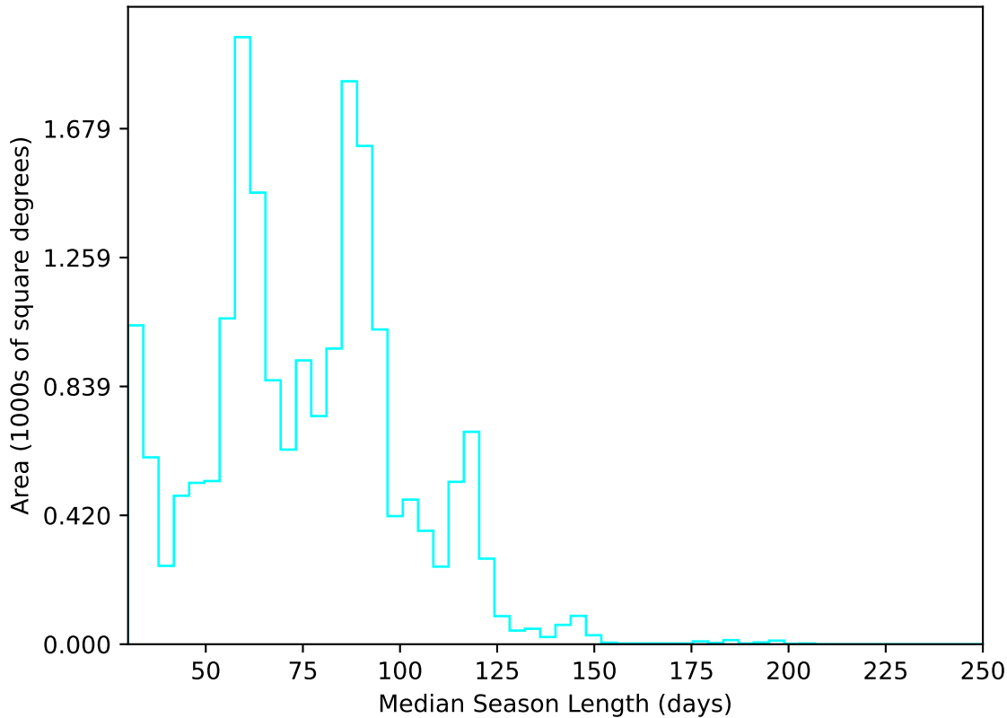
too_elab_r256_d2_ugrizy_v3.4_10yrs All sky u band: Median Season Length
