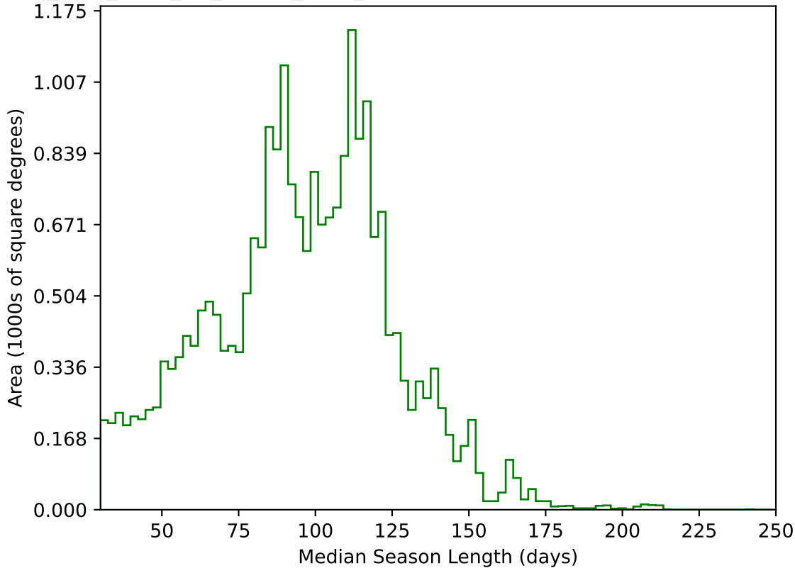
too_elab_r256_d2_ugrizy_v3.4_10yrs All sky g band: Median Season Length
