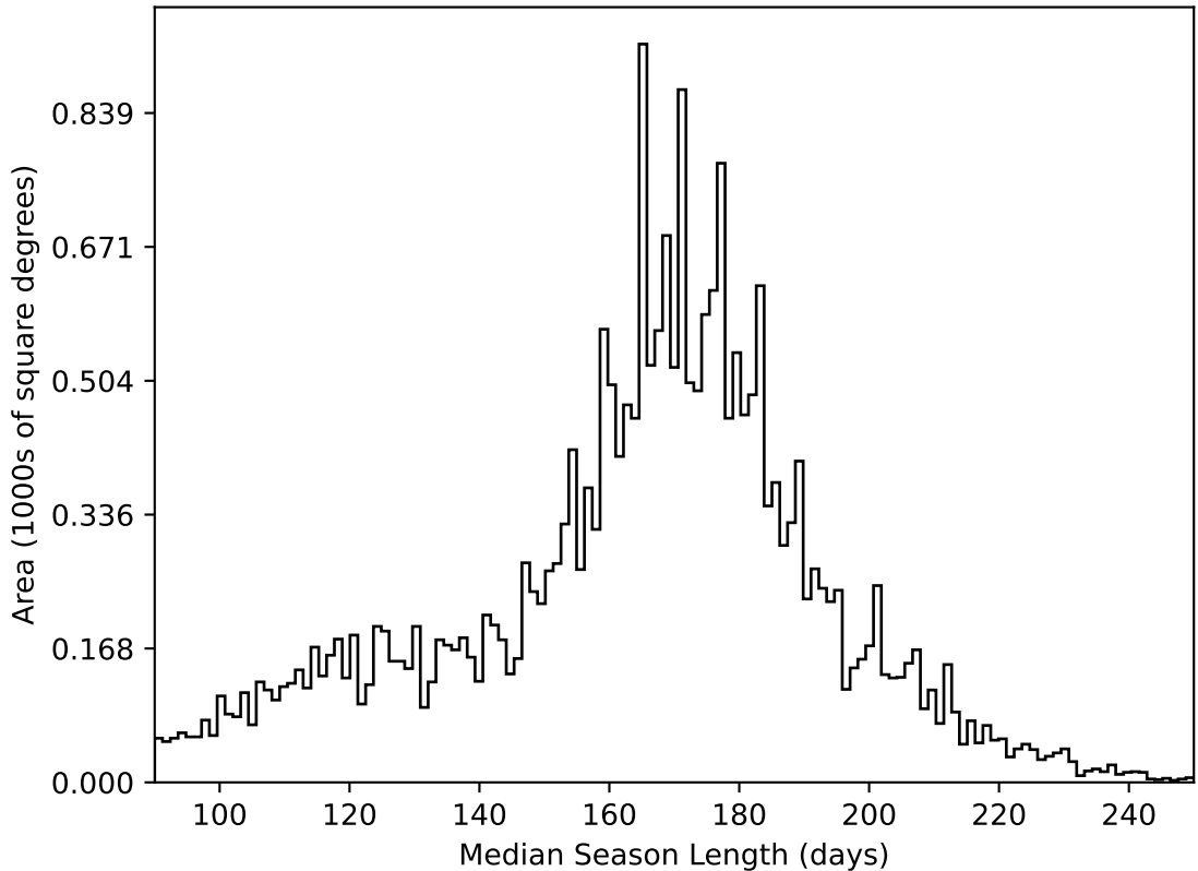
too_elab_r256_d2_ugrizy_v3.4_10yrs All sky all bands: Median Season Length
