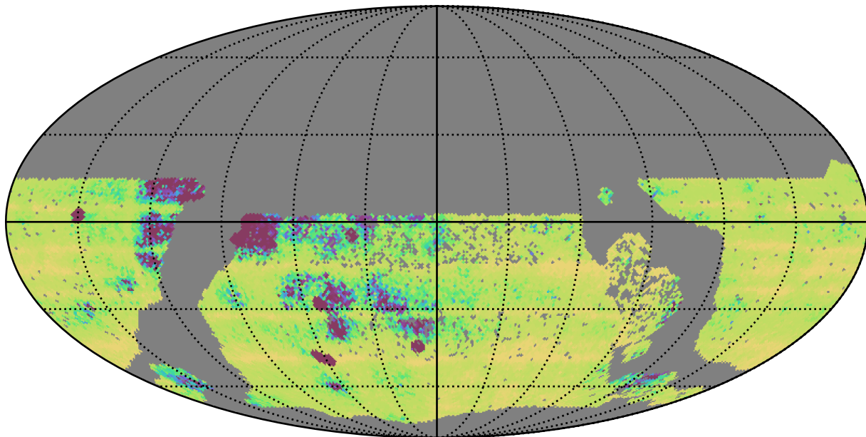
too_elab_r256_d2_ugrizy_v3.4_10yrs WFD: Median Intra-Night Gap
