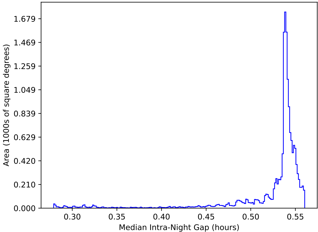
too_elab_r256_d2_ugrizy_v3.4_10yrs WFD: Median Intra-Night Gap
