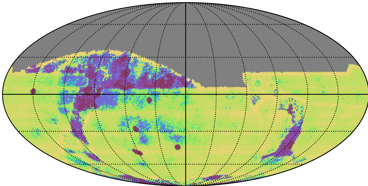
too_elab_r256_d2_ugrizy_v3.4_10yrs All sky: Median Intra-Night Gap
