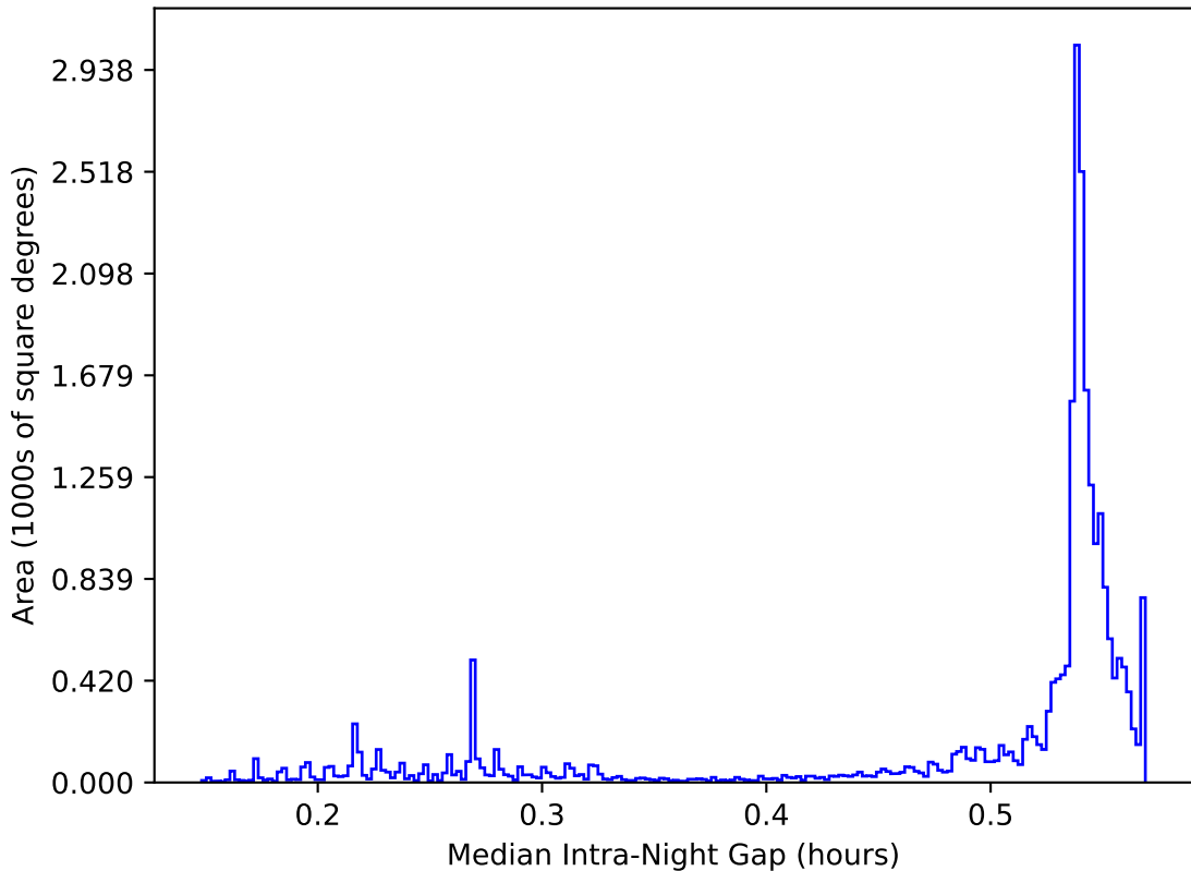
too_elab_r256_d2_ugrizy_v3.4_10yrs All sky: Median Intra-Night Gap
