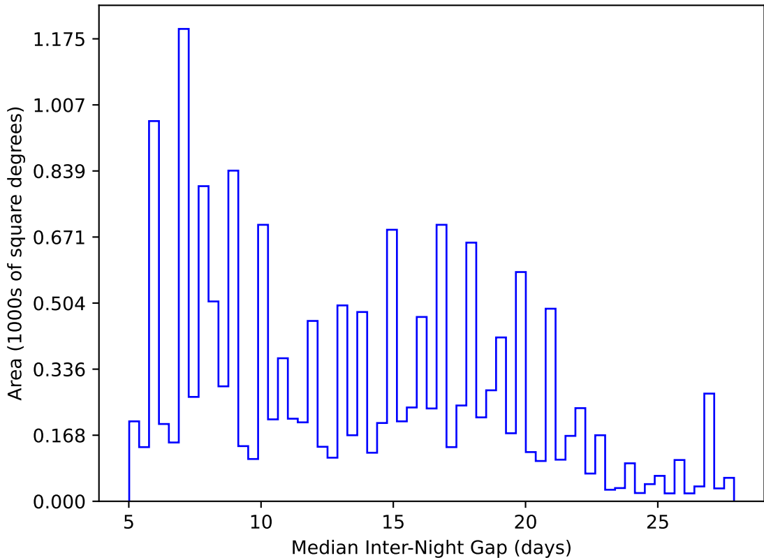
too_elab_r256_d2_ugrizy_v3.4_10yrs WFD y band: Median Inter-Night Gap
