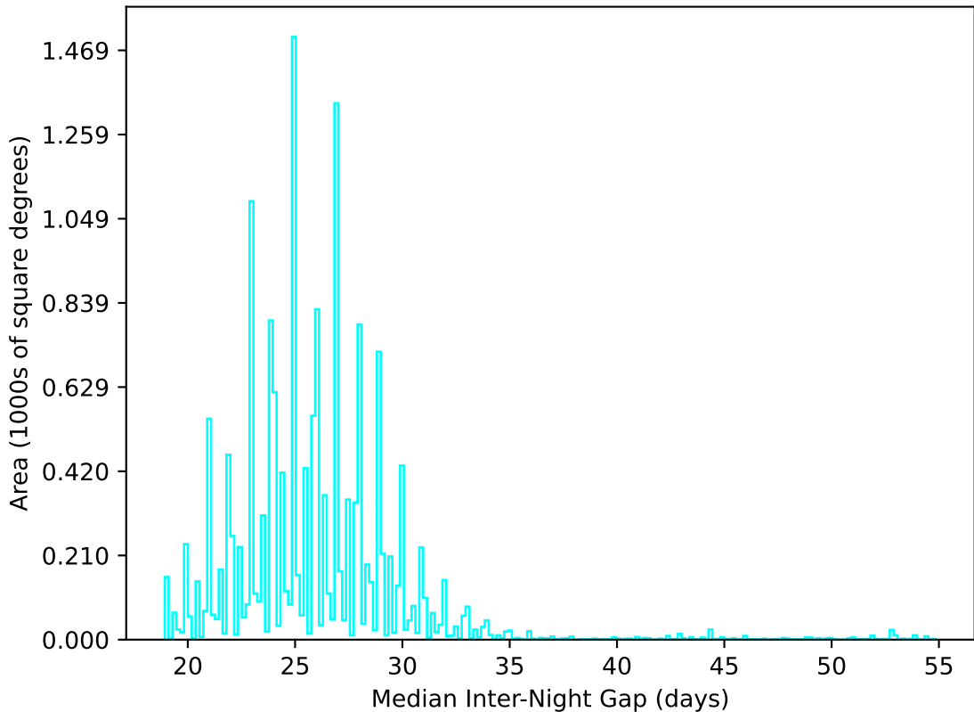
too_elab_r256_d2_ugrizy_v3.4_10yrs WFD u band: Median Inter-Night Gap
