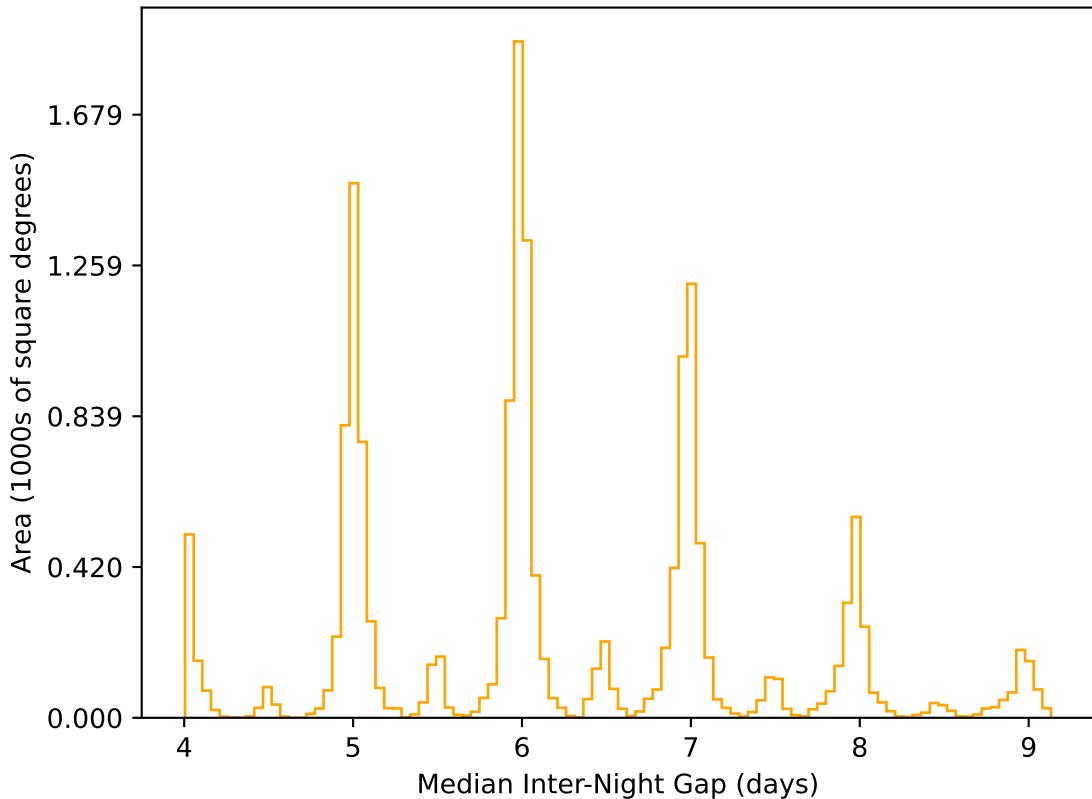
too_elab_r256_d2_ugrizy_v3.4_10yrs WFD r band: Median Inter-Night Gap
