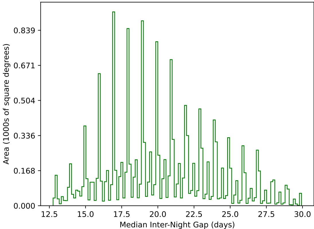
too_elab_r256_d2_ugrizy_v3.4_10yrs WFD g band: Median Inter-Night Gap
