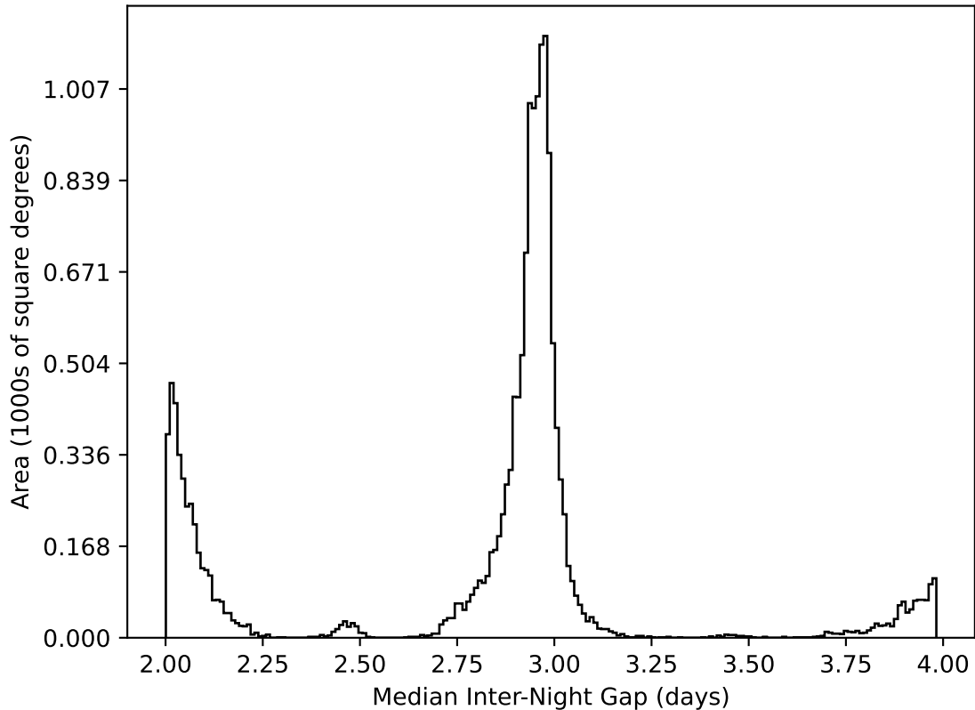
too_elab_r256_d2_ugrizy_v3.4_10yrs WFD all bands: Median Inter-Night Gap
