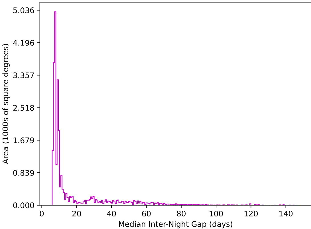
too_elab_r256_d2_ugrizy_v3.4_10yrs All sky z band: Median Inter-Night Gap
