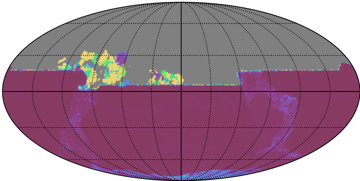
too_elab_r256_d2_ugrizy_v3.4_10yrs All sky y band: Median Inter-Night Gap
