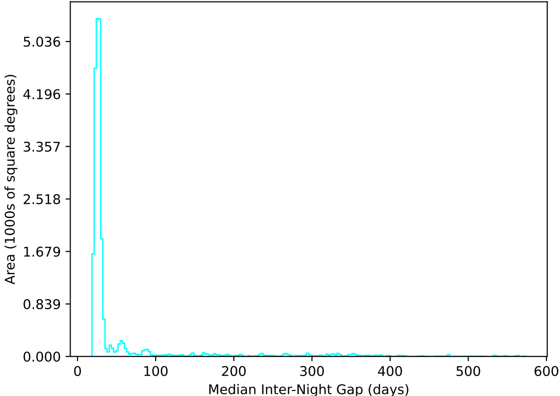
too_elab_r256_d2_ugrizy_v3.4_10yrs All sky u band: Median Inter-Night Gap
