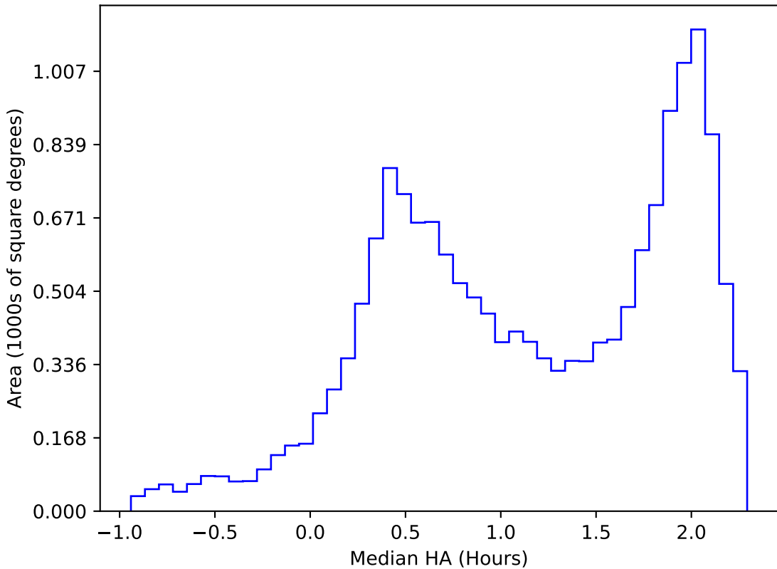
too_elab_r256_d2_ugrizy_v3.4_10yrs WFD z band: Median HA
