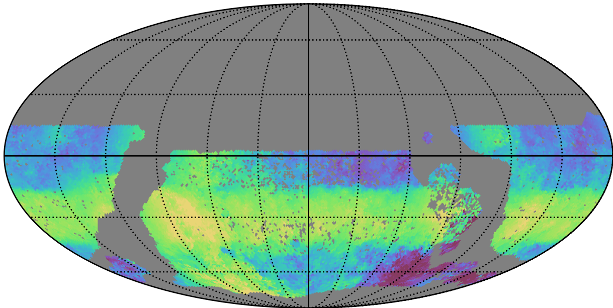
too_elab_r256_d2_ugrizy_v3.4_10yrs WFD u band: Median HA
