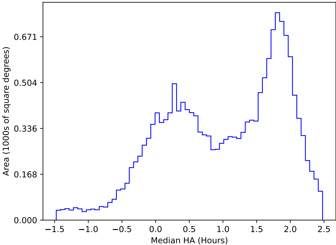
too_elab_r256_d2_ugrizy_v3.4_10yrs WFD u band: Median HA
