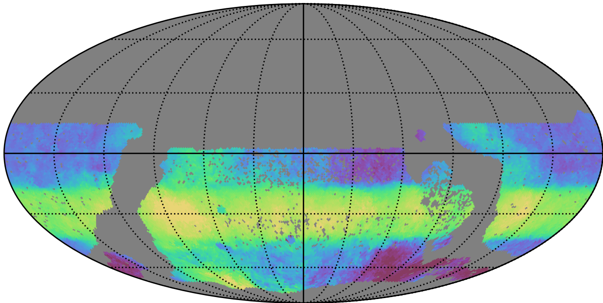
too_elab_r256_d2_ugrizy_v3.4_10yrs WFD r band: Median HA
