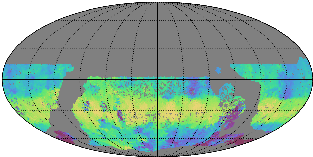
too_elab_r256_d2_ugrizy_v3.4_10yrs WFD g band: Median HA
