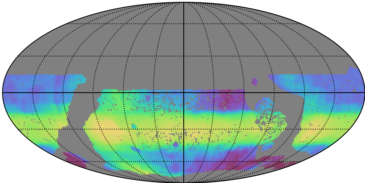
too_elab_r256_d2_ugrizy_v3.4_10yrs WFD all bands: Median HA
