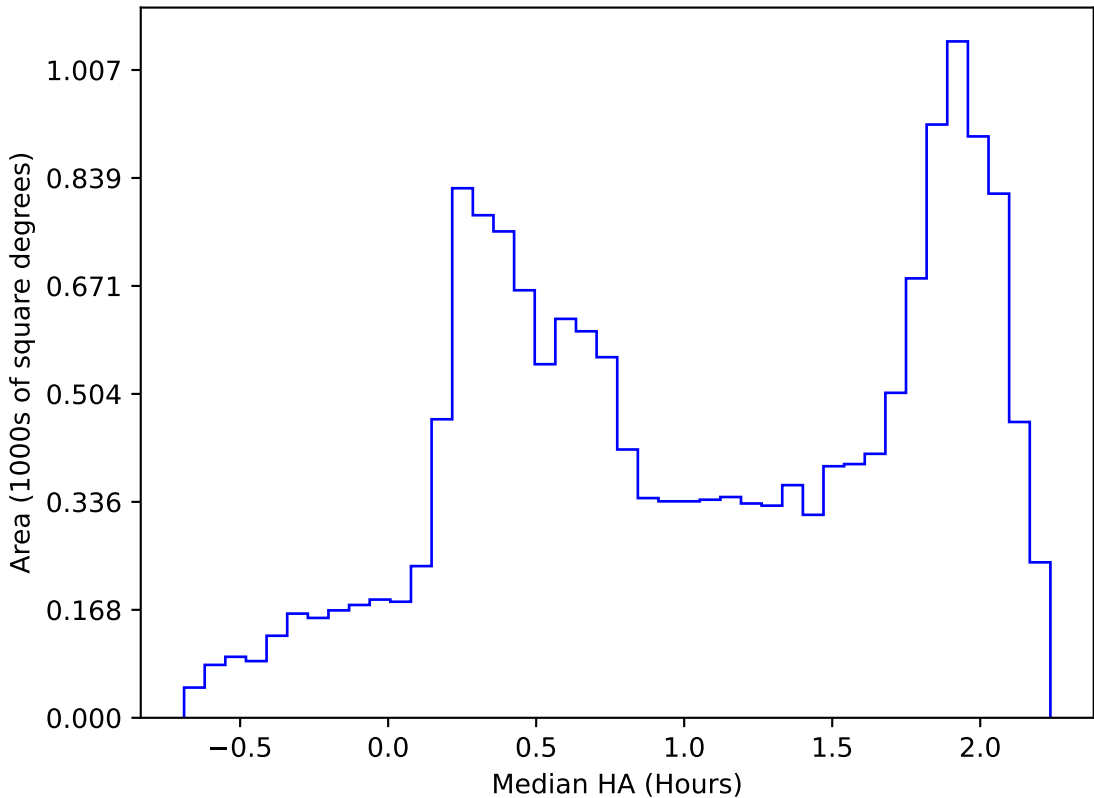
too_elab_r256_d2_ugrizy_v3.4_10yrs WFD all bands: Median HA
