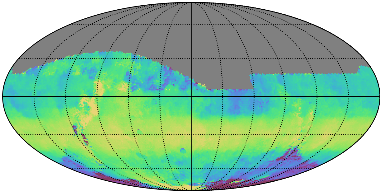
too_elab_r256_d2_ugrizy_v3.4_10yrs All sky z band: Median HA
