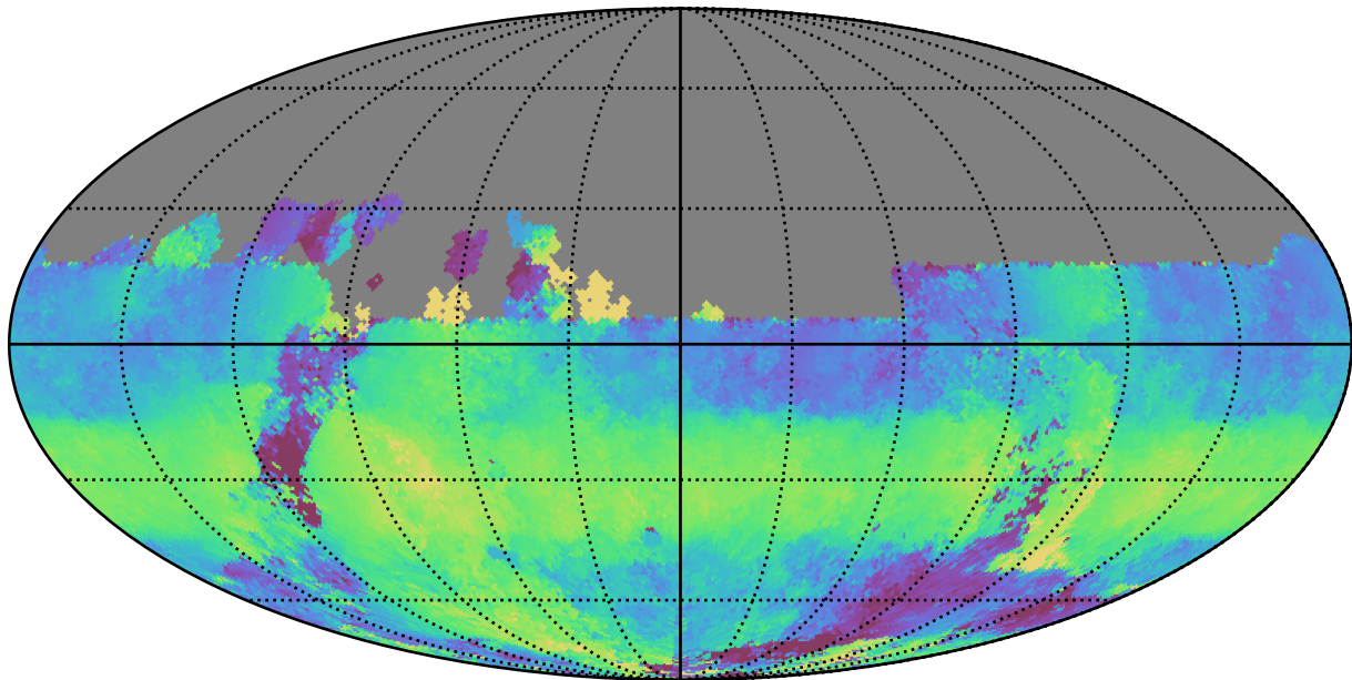
too_elab_r256_d2_ugrizy_v3.4_10yrs All sky u band: Median HA
